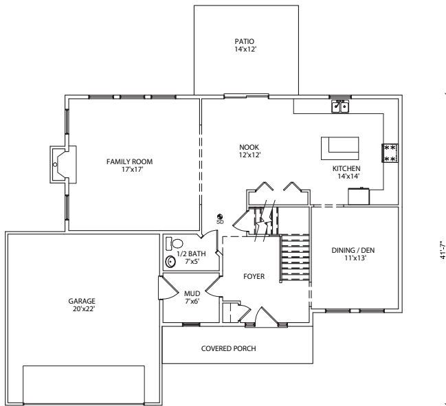
FIRST FLOOR PLAN BELLMORE SPEC
