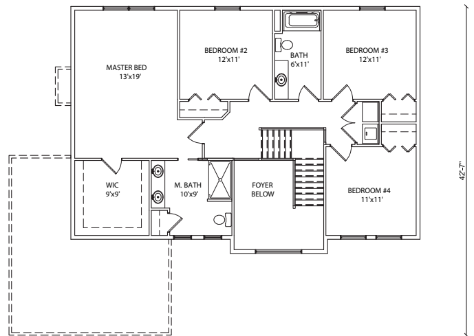
SECOND FLOOR PLAN BELLMORE SPEC
